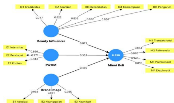
Figure 1. Algorithm Model
