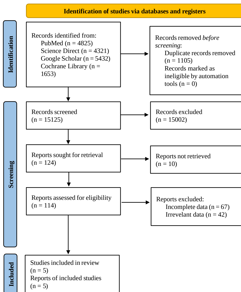
Figure 1. PRISMA Flowchart
